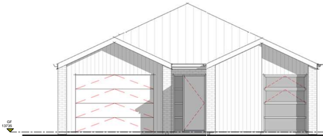
1 EAST ELEVATION 1 : 50 12M HEIGHT
