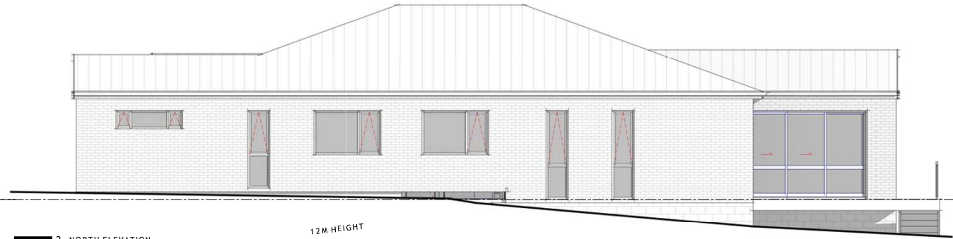
2 NORTH ELEVATION 1 : 50 12M HEIGHT
