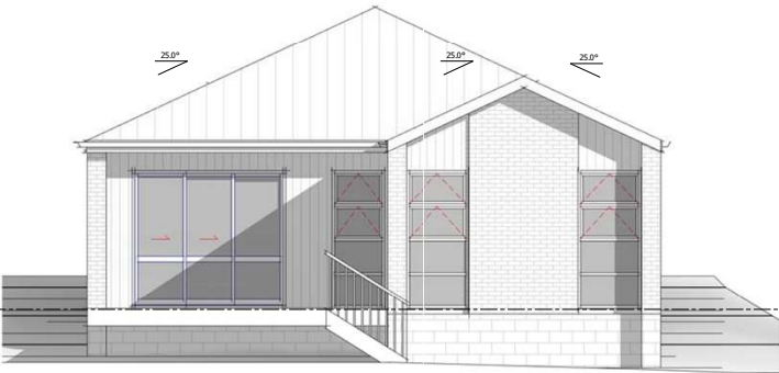
3 WEST ELEVATION 1 : 50
